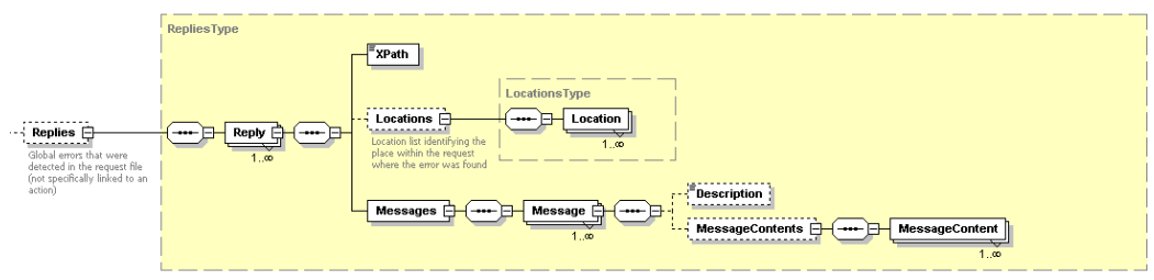
Figure 31: Replies Tag Structure
