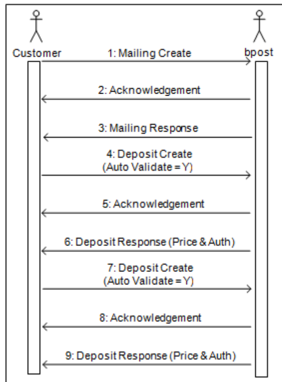
Figure 25: Mailing file, multiple deposits (Auto Validate = Y)
