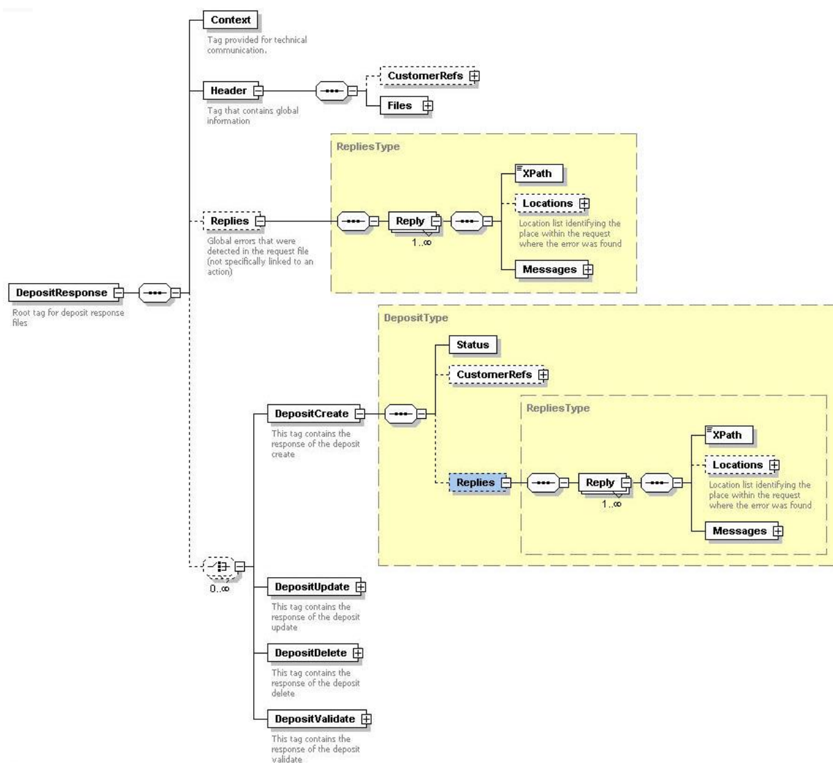
Figure 30: DepositResponse File Structure
