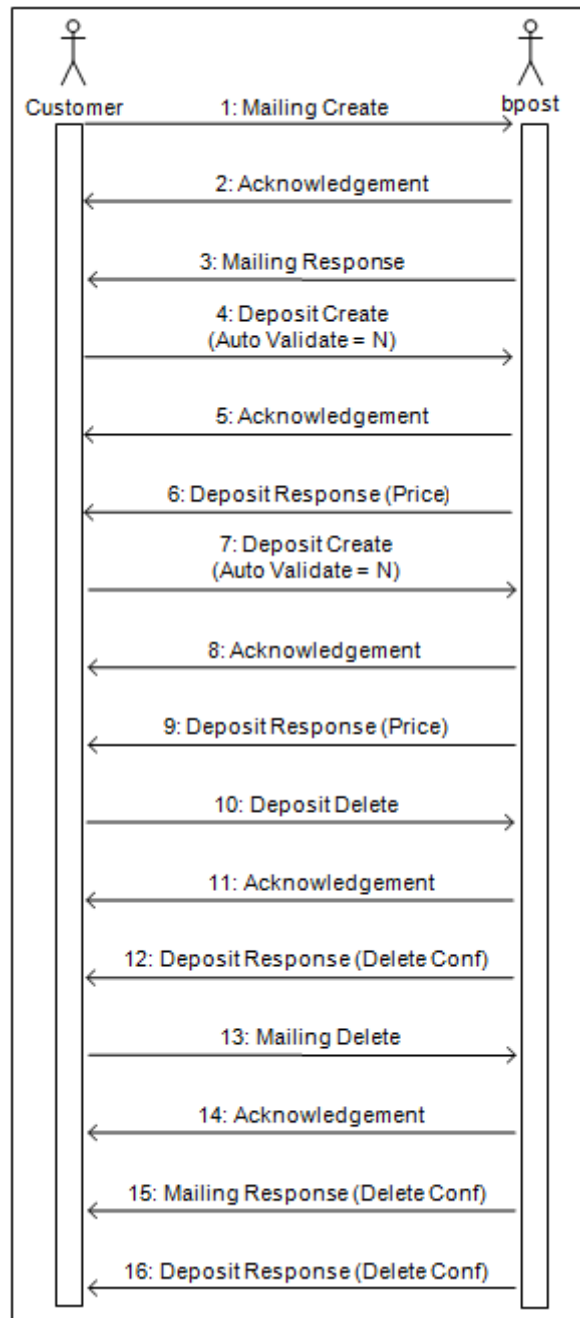
Figure 26: Mailing file Delete
