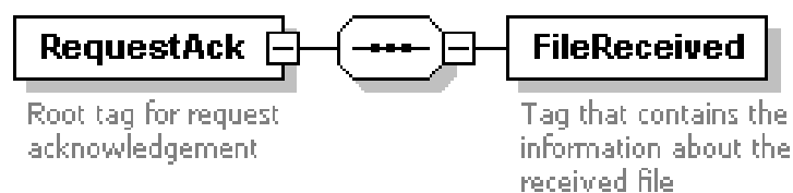
Figure 33: Mailing Acknowledgement File Structure
